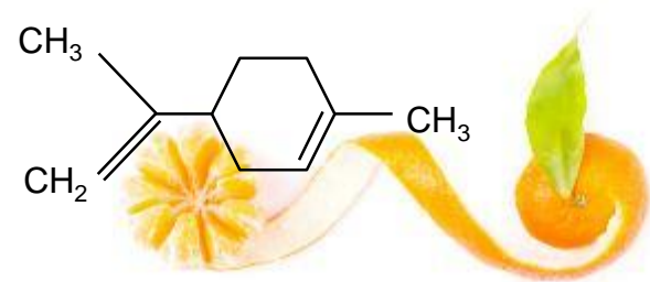
D-Limonene
